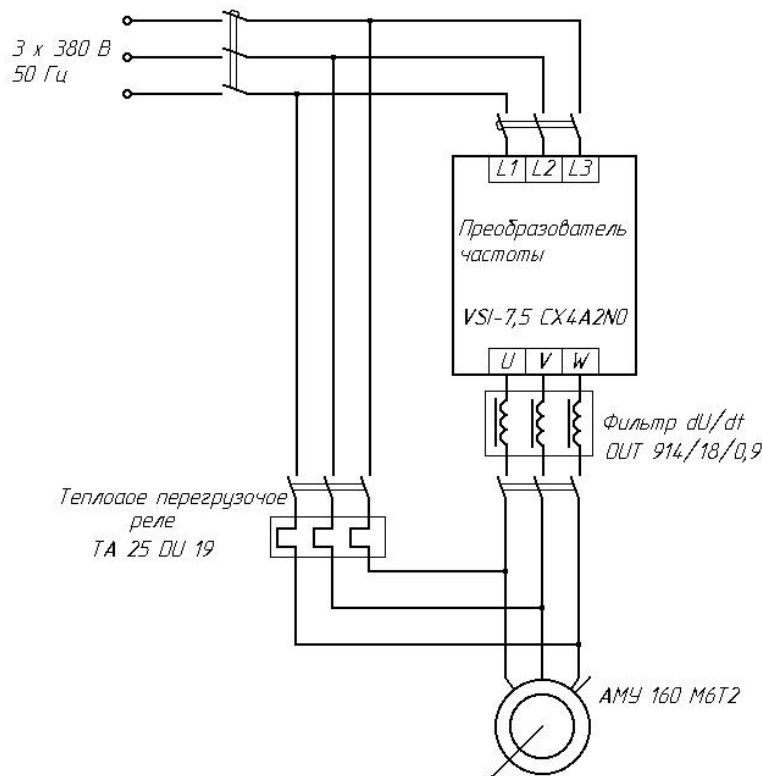
Structural diagram of the drive power unit
