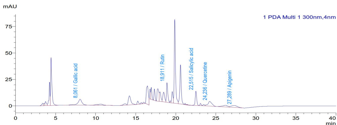
Figure 2. Chromatogram for the determination of polyphenols in the sample extract.
