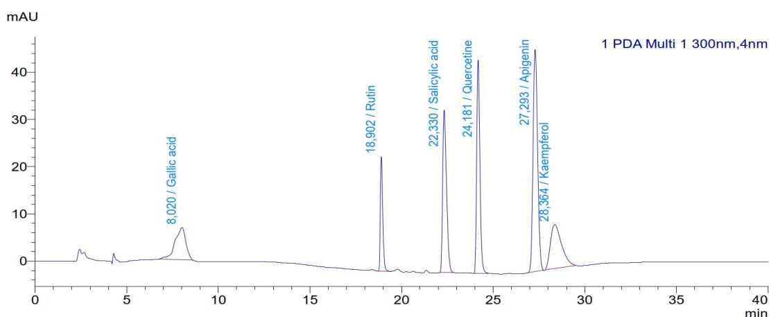
Figure 1. Chromatogram of standards at 300 nm
